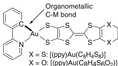
Scheme 1 Schematic drawing of unsymmetrical organometallic donors
