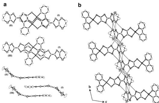
Fig. 5 (a) Molecular arrangements viewed along the molecular planes. (b) Packing diagram viewed along the bc plane in [(ppy)Au(C 8 H 4 S 8 )]. Fine lines show sulfur-sulfur contacts (<3.7 Å) (Reprinted with permission from [26]. Copyright 2003 Elsevier)
