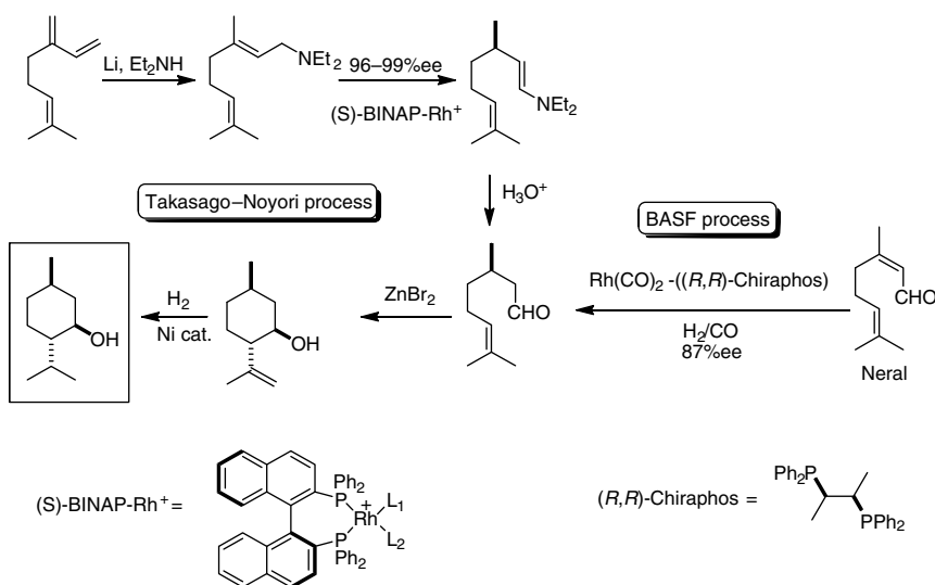
SCHEME 1.1 Industrial menthol processes.
