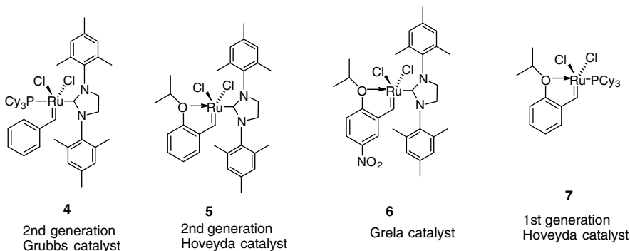
FIGURE 1.9 RCM catalysts.
