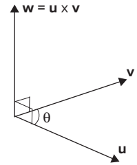
FIGURE 1-20: The geometry used in the cross product
