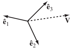
Figure 1.1: An orthonormal set of unit vectors \hat{\mathbf{e}}_1, \hat{\mathbf{e}}_2, \hat{\mathbf{e}}_3 . \mathbf{V} is an arbitrary vector.
