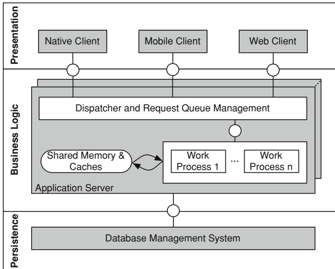
Fig. 2.2 Three-tier architecture of SAP R/3
