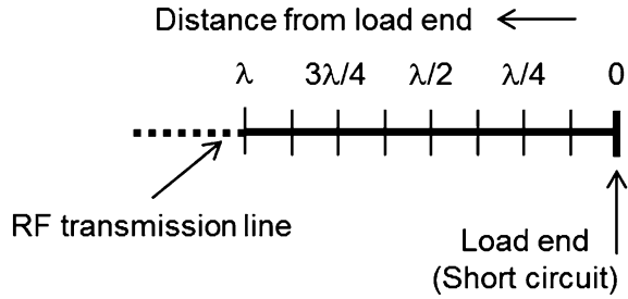
Fig. 2.9 RF transmission line—short circuit
