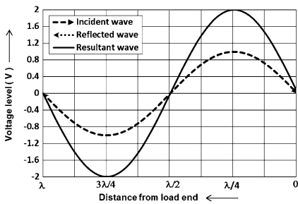
Fig. 2.10e t = \lambda/2 for short circuited line
