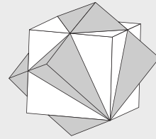
Fluorit-Kristall
