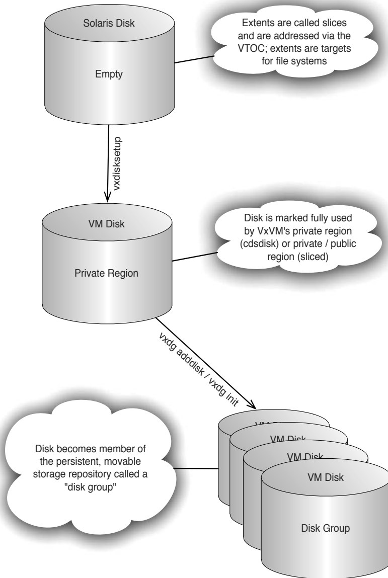
Figure 2-1: Initializing a disk for VxVM creates a so-called VM disk, which is marked "completely full" for the operating system (but not for VxVM). It can then be added to a disk group using the appropriate command, and subsequently used as persistent backing store for virtual volumes.
