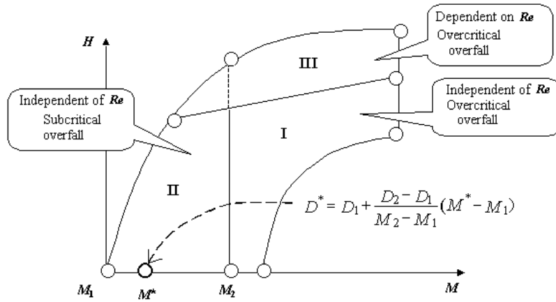
Figure 2.3. Adaptation of controller to flight conditions
