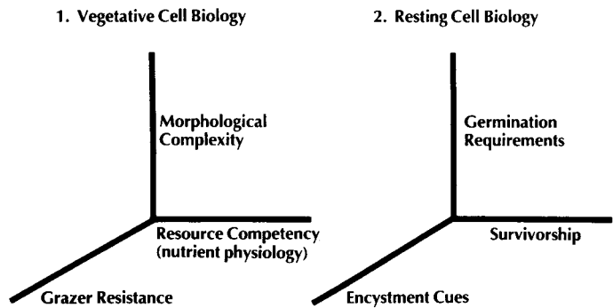
Fig. 1-1. Interacting aspects of phytoplankton population and reproductive ecology that compose the elements of a planktonic alga's life history strategy. (A) Typical life history for many phytoplankton species exhibiting an alternation between vegetative cells and resting cells (resting cyst in this example). (B) Axes representing the characteristics by which microalgae diversify and adapt for persistence in stressful, heterogeneous planktonic habitats.
