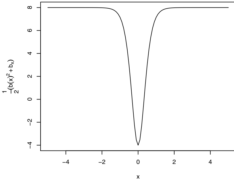
Fig. 2.4. Graph of the curve \frac{1}{2}(b(x)^2 + b_x(x)) .
