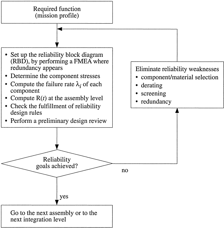
Figure 2.1 Reliability analysis procedure at assembly level
