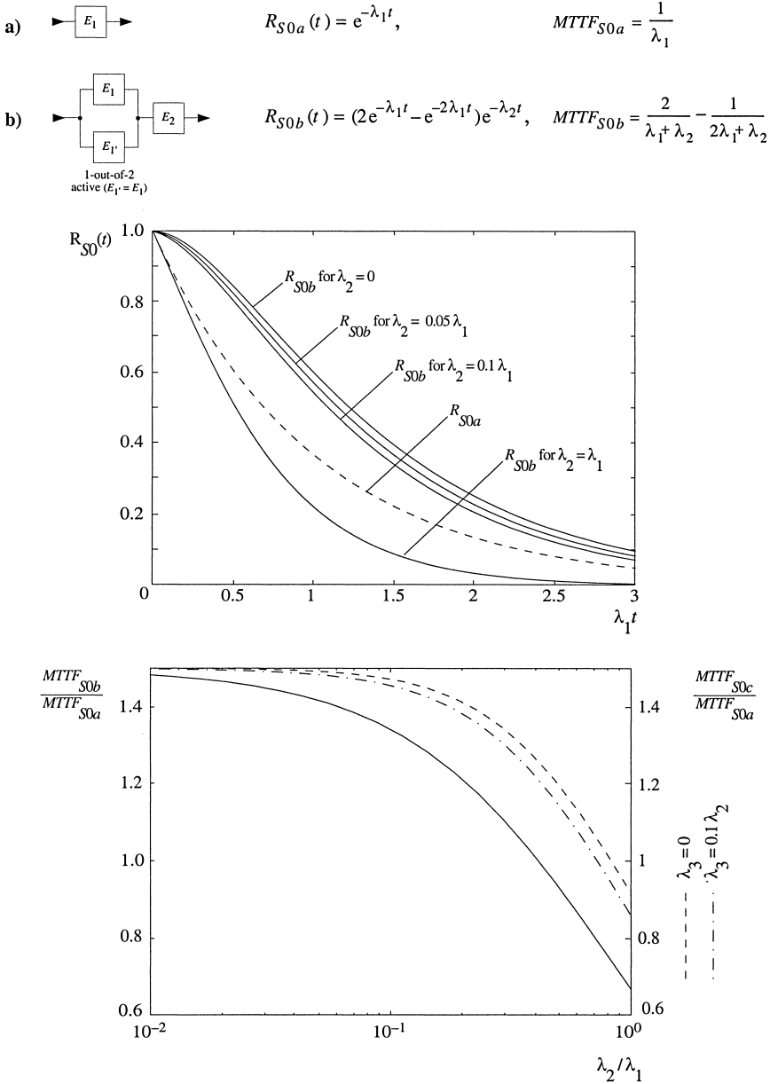
Figure 2.8 Comparison between the one-item structure and a 1-out-of-2 active redundancy with series element (nonrepairable up to system failure, independent elements, constant failure rates \lambda_1 & \lambda_2 , \lambda_1 remains the same in both structures; equations according to Table 2.1; given on the right-hand side is MTTF_{S0c} / MTTF_{S0a} with MTTF_{S0c} from Fig. 2.9; see Fig. 6.17 for the repairable case)
